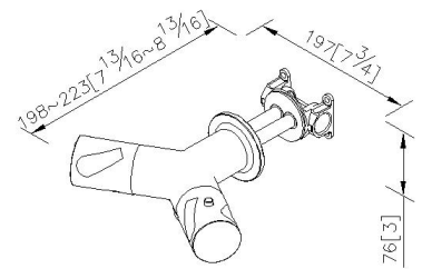
unit: mm[inch]
